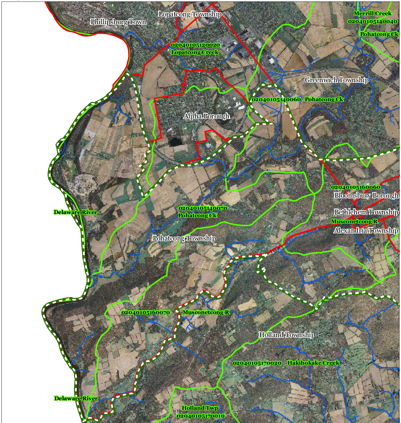
Figure 3: HUC 14 Boundaries
