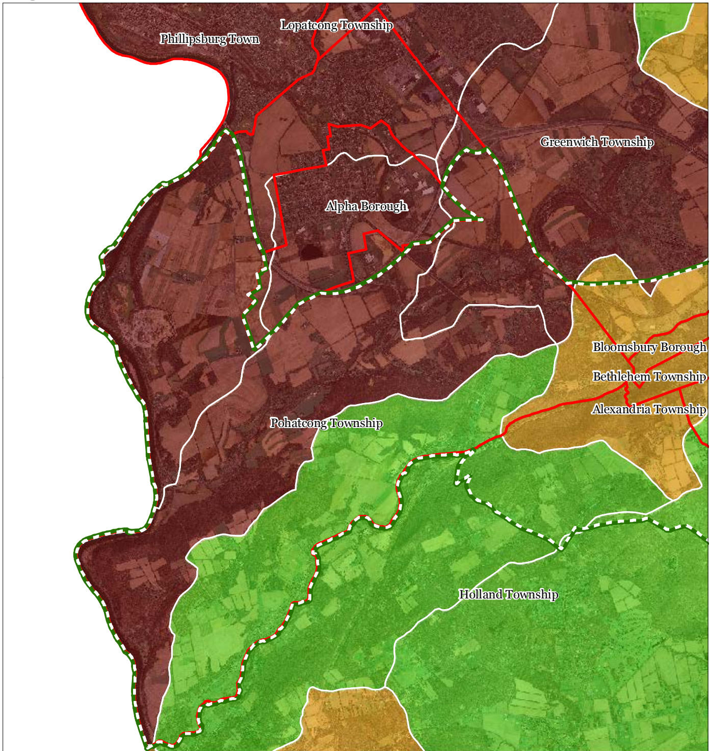
Figure 6: Forest Subwatersheds
